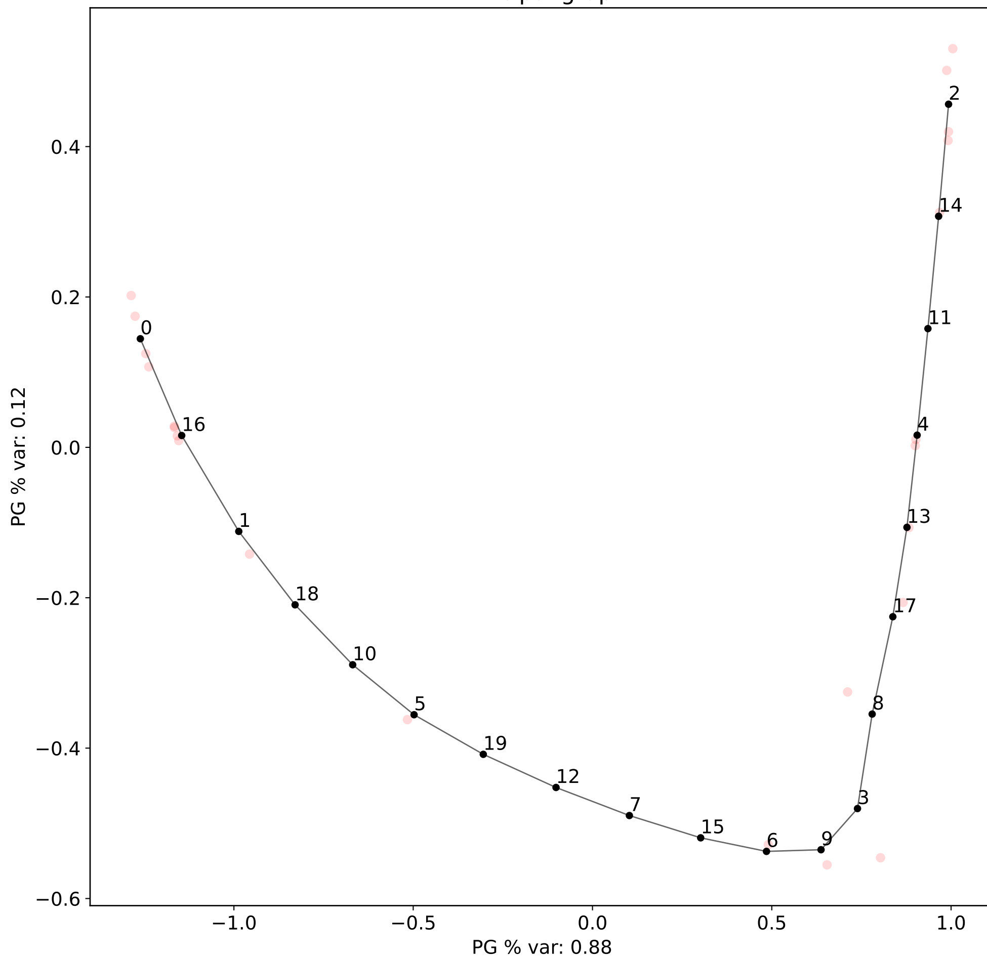
Principal graph
